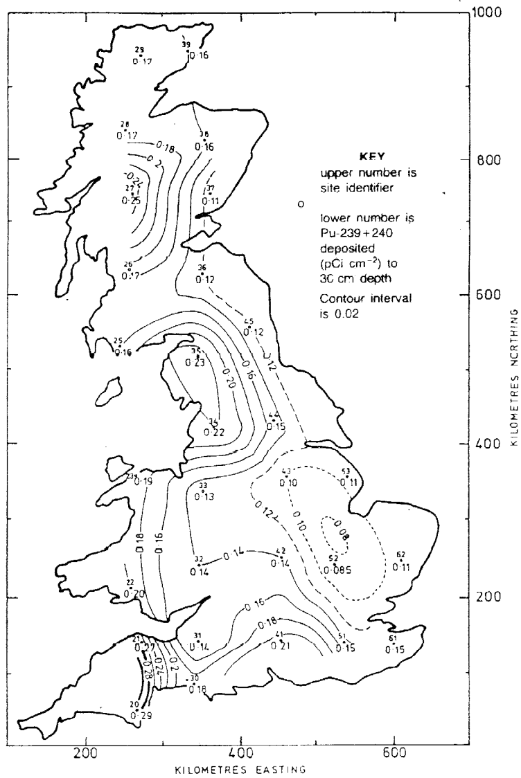
AERE R 10155 Fig. 4.6 Woodland 1977: deposition of Pu-239+240 in soil to 30 cm depth
