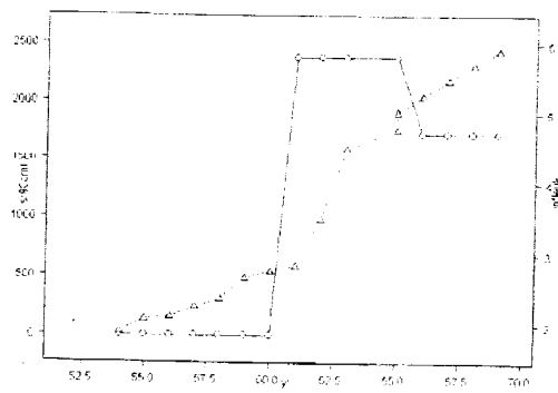
Fig 1 Infant leukemia in Denmark by 5-yr aggregates from 1952 to 1970 (-o-) with cumulative dose from Sr-90 to adults over the same period (-Δ-).
