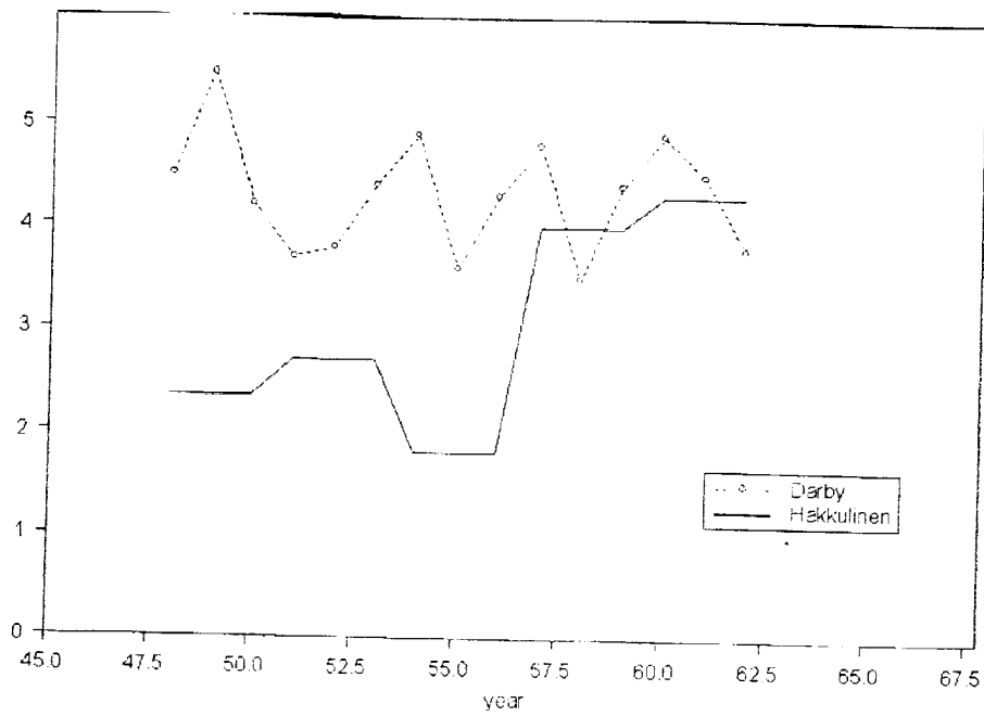
Fig 2 Childhood leukemia rates 0-14 in Denmark according to Darby et al. 1993 and Hakkulinen et al. 1986. Hakkulinen rates are aggregates of three-year groups.
