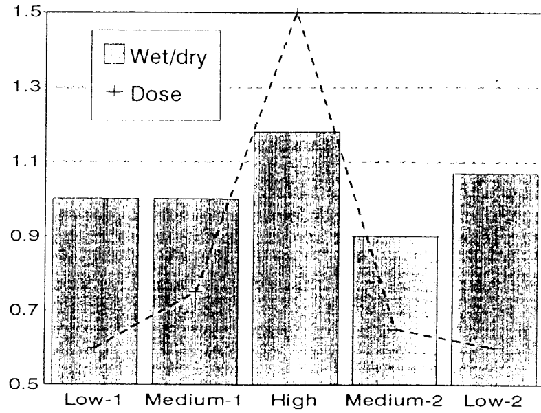
FIG.5.3. Fallout and childhood leukemia age 0-4.
